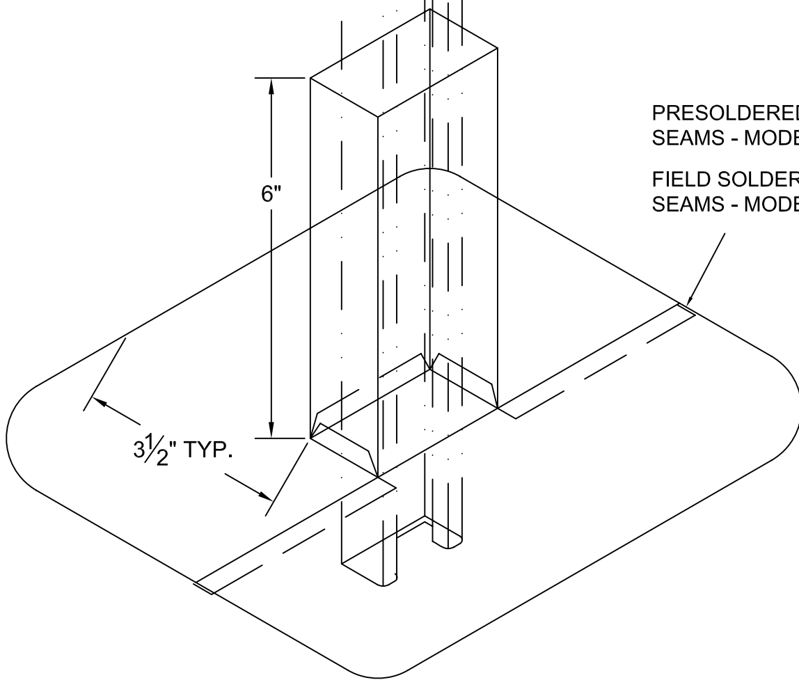
STRUT FLASHING - Models U/D and U/S
